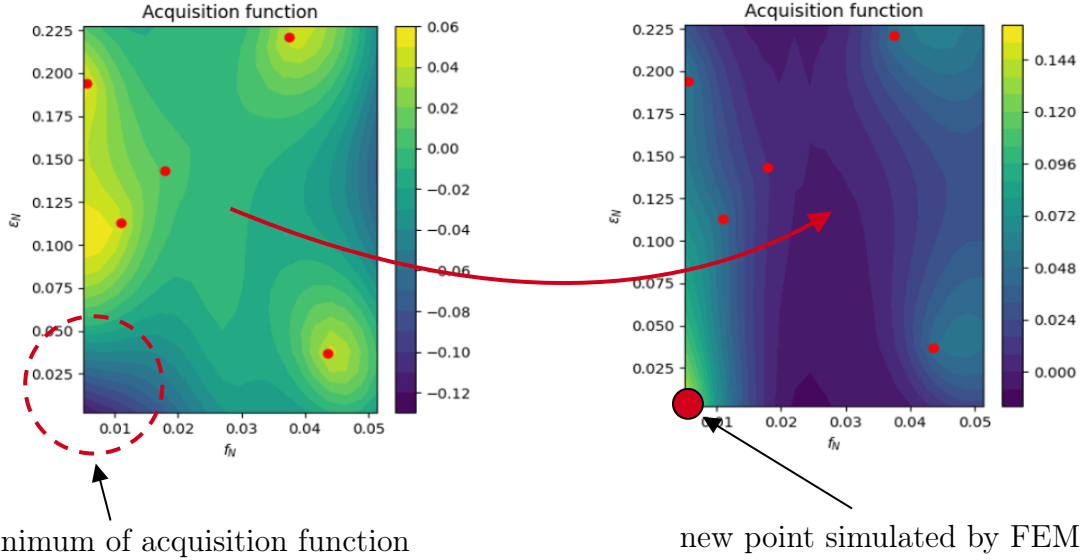
Figure 2: Choice of the new pair of GTN parameter f_N and \epsilon_N for an additional FEM simulation.
